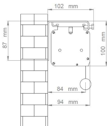
Wall mounting, front unrolling
