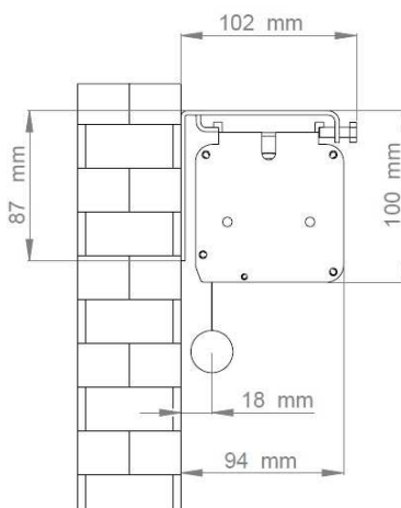
Wall mounting, back unrolling
