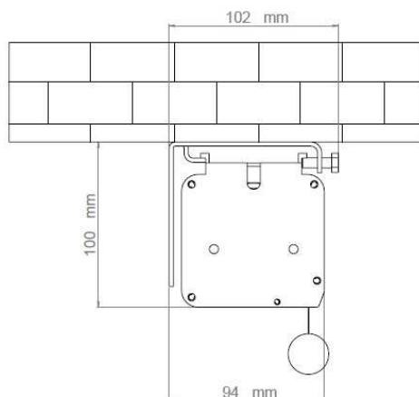
Ceiling mounting
