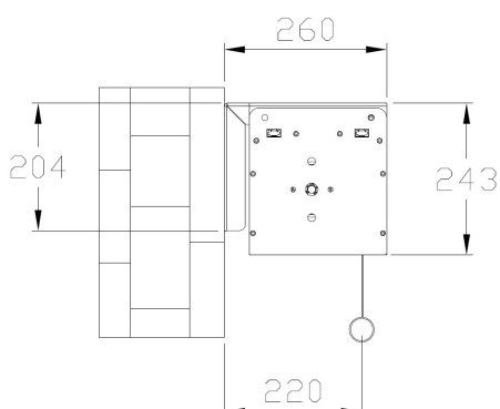
Wall mounting- front unrolling
