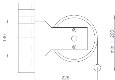
Wall mounting- front unrolling
