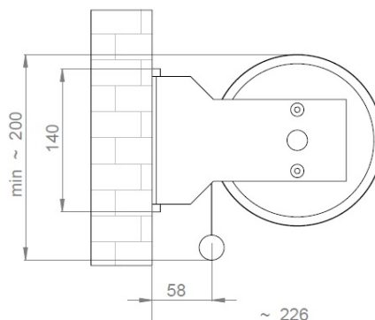
Wall mounting- back unrolling
