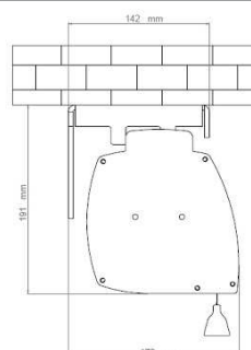
Ceiling mounting
