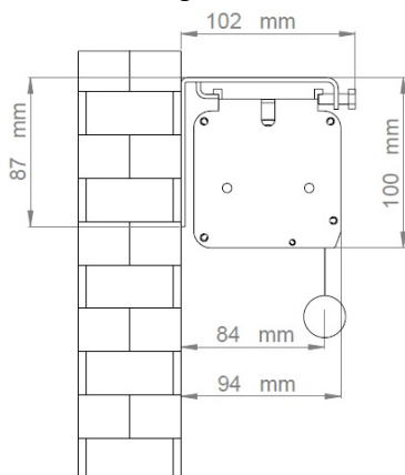
Wall mounting
