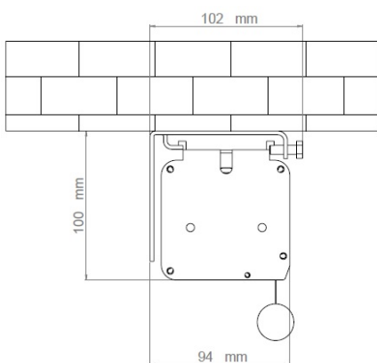
Ceiling mounting
